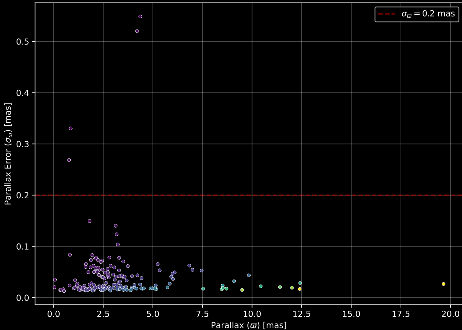
APOGEE DR17 Field: [K2_C3_042-56] Parallax Quality (n= 176)
