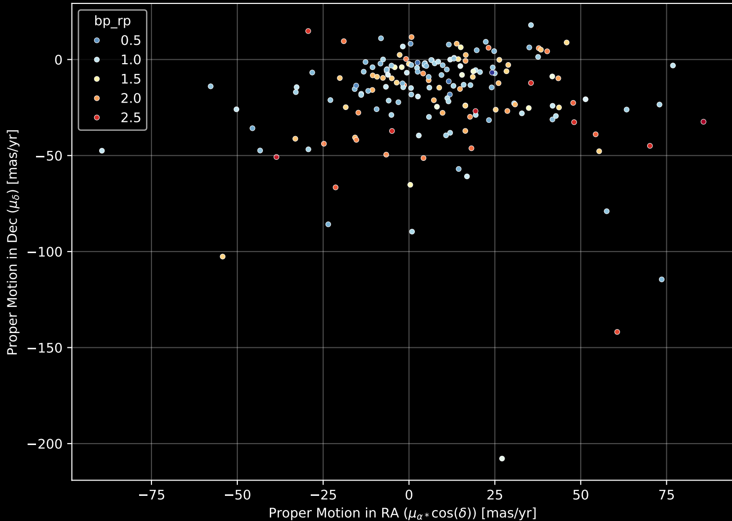
APOGEE DR17 Field: [K2_C3_042-56] Proper Motion Diagram (n= 176)
