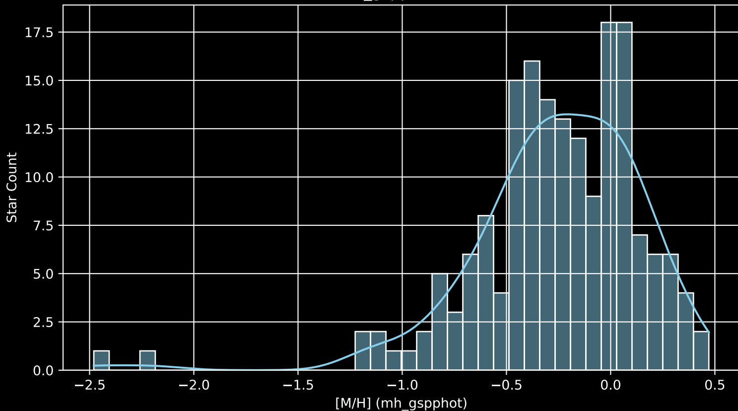
APOGEE DR17 Field: [K2_C3_042-56 [M/H] (mh_gspphot) (n= 176)
