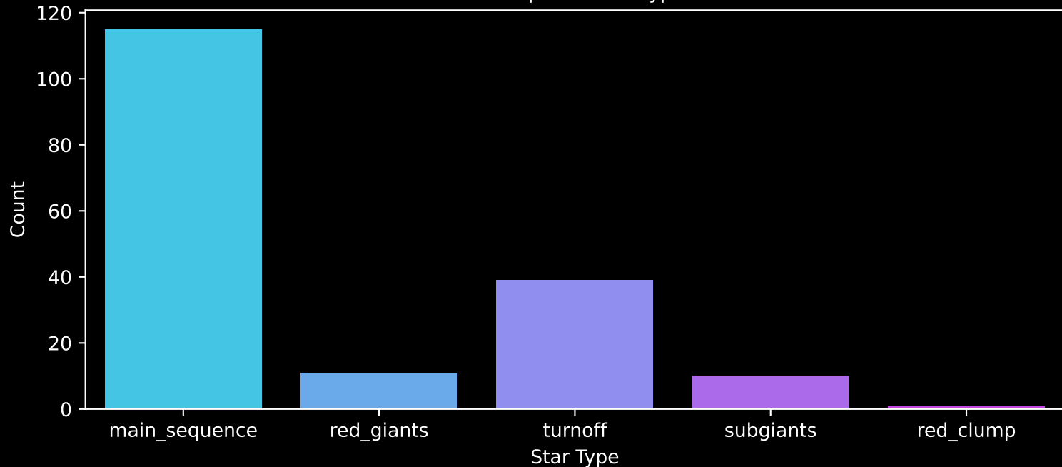
APOGEE DR17 Field: [K2_C3_042-56] Count plot of Star Type
