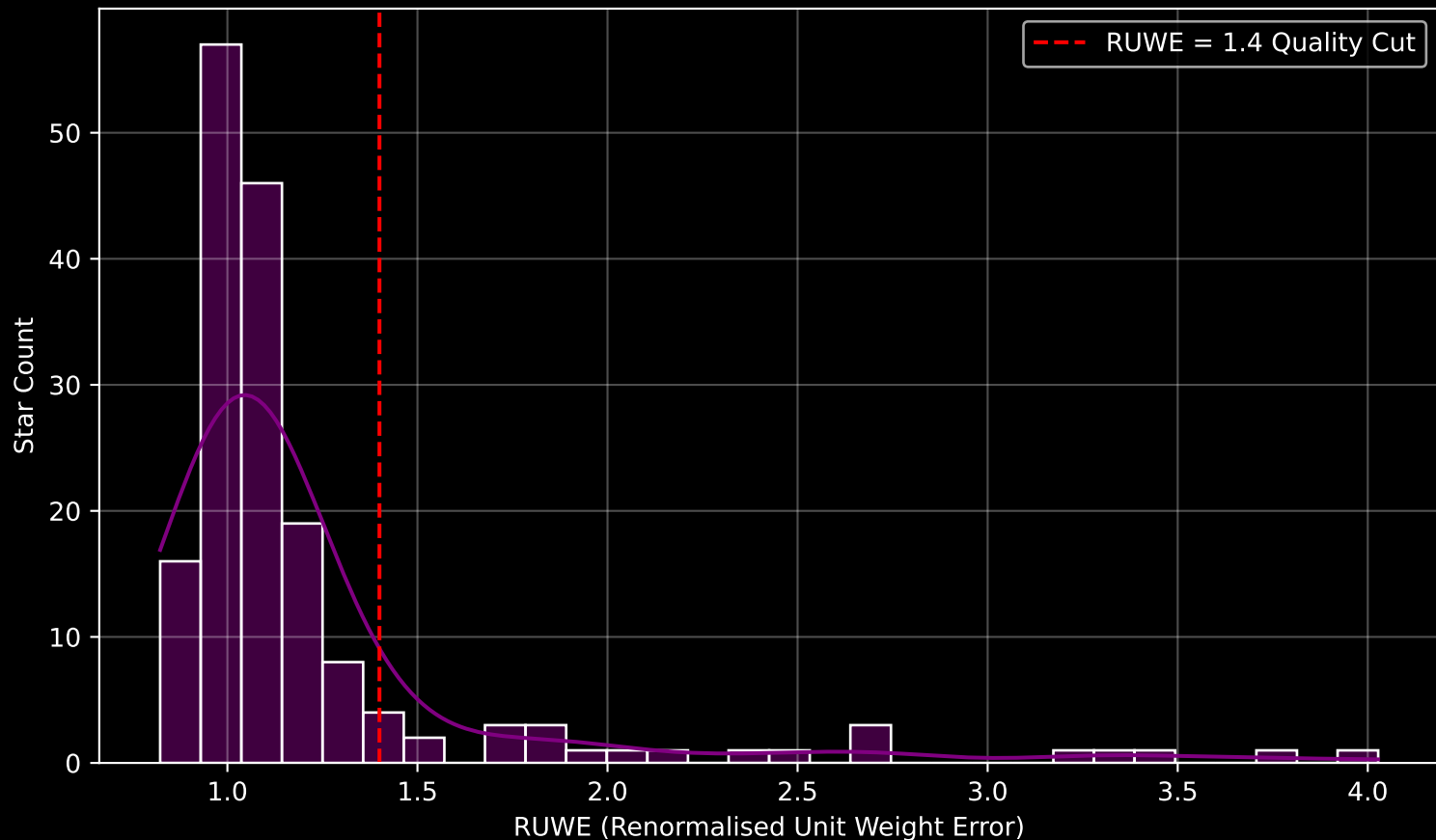
GAPOGEE DR17 Field [K2_C3_042-56] RUWE Distribution (n= 171)
