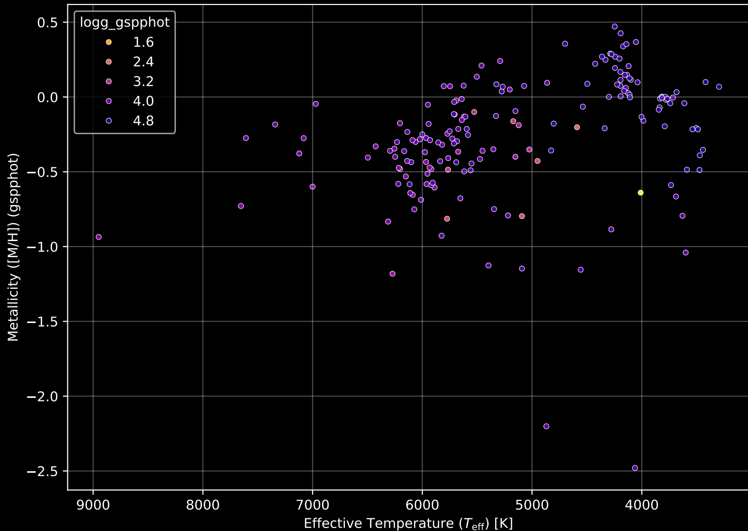
APOGEE DR17 Field: [K2_C3_042-56] Stellar Population Parameters (n= 176)
